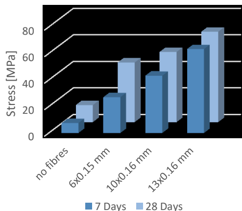
Figure 5: Flexural strength for different fibre types.
