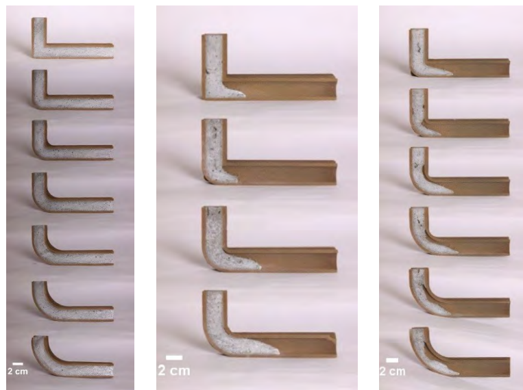
Figure 4: L-shaped tubes with varying bending radii: Left 6 x 0.15mm fibres; middle 10 x 0.16mm fibres; right 13 x 0.16mm fibres. Bending radii (left picture), from top to bottom [mm]: 0, 10, 20, 30, 40, 50, 60. Arms on both sides of each L-shaped tube were originally 15 cm long.
