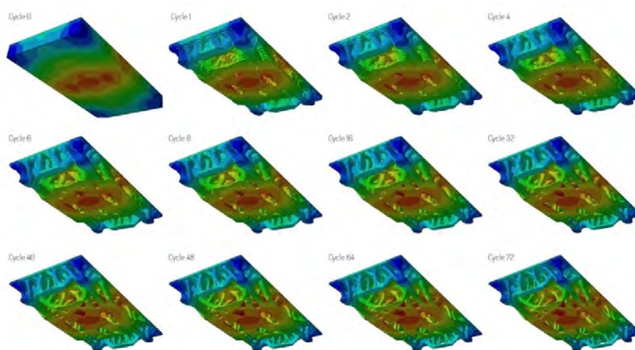
Figure 3: Topology optimisation iterations for the slab prototype
